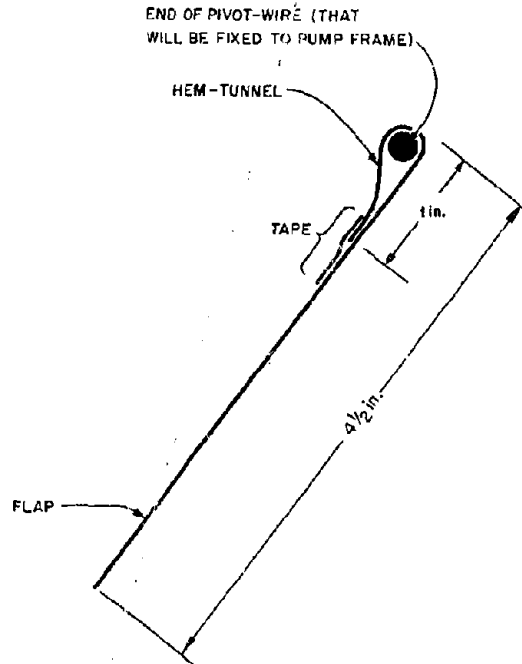
Fig. B-8. End view of flap.
